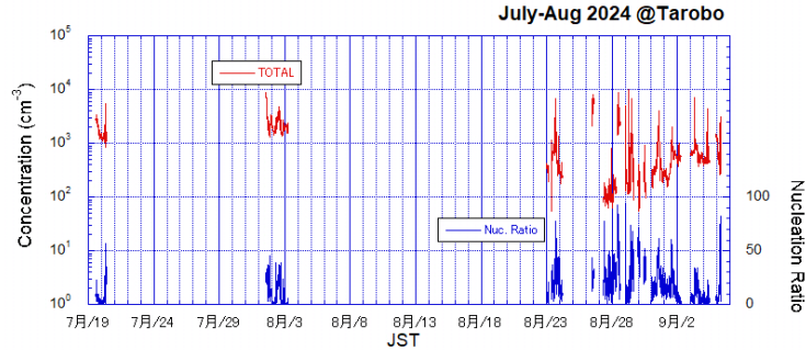
Fig. 1 Total particle concentration and ratio of nucleation modes measured at Tarobo during the 2024 summer intensive observation.
